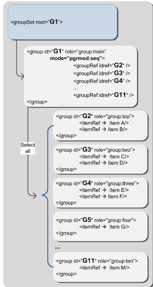
Code skeleton of a sequential mode package and (right) the resulting relationship structure
