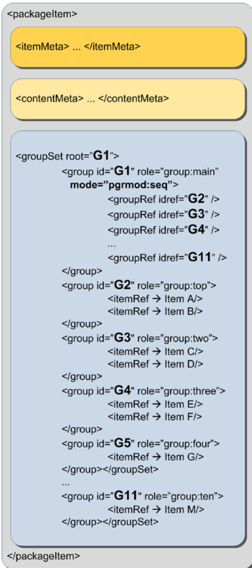
Code skeleton of a sequential mode package and (right) the resulting relationship structure
