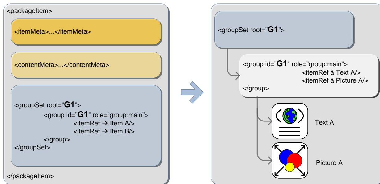
Top-level element view of a simple package, and (right) a visualisation of the structure
