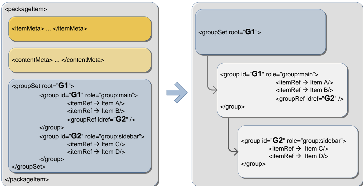
Code outline of hierarchical package with two groups visualising the parent-child structure (right)
