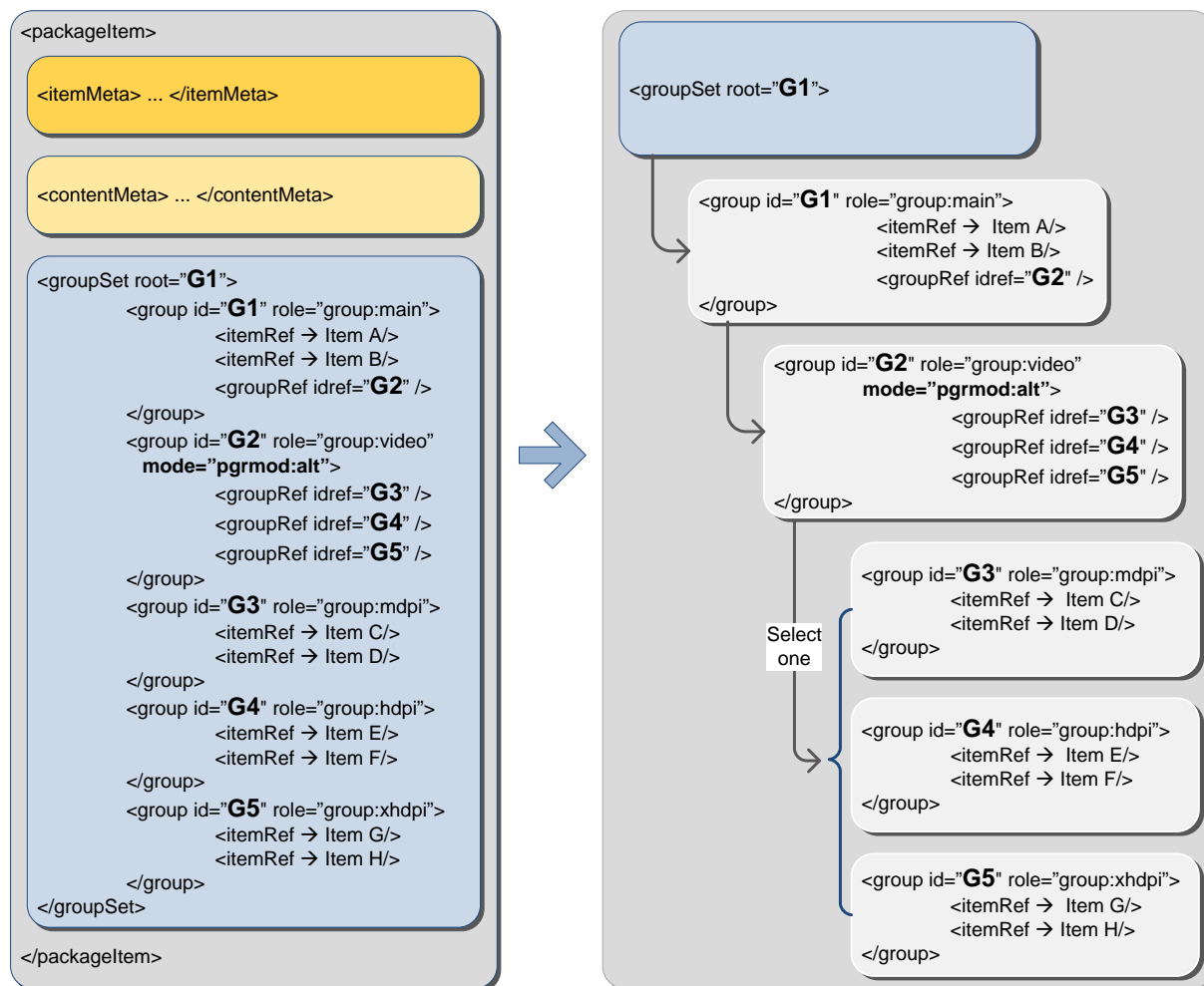
Code skeleton view of a package with alternative components, with a visual representation of the structure
