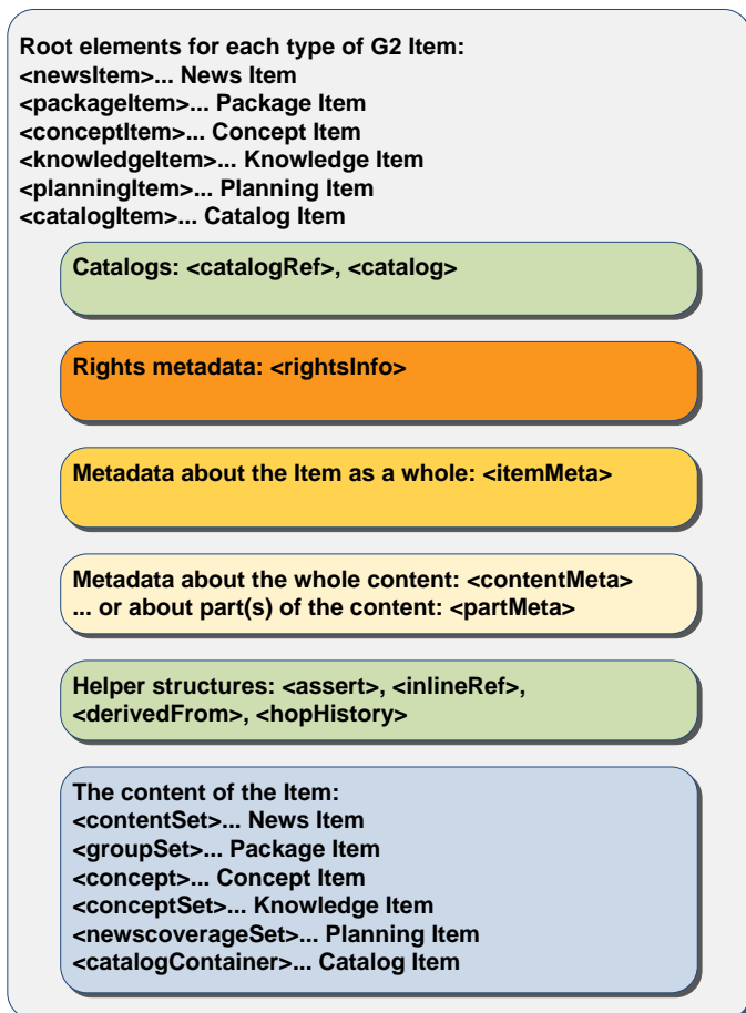
The basic XML elements associated with each part of a G2 Item
